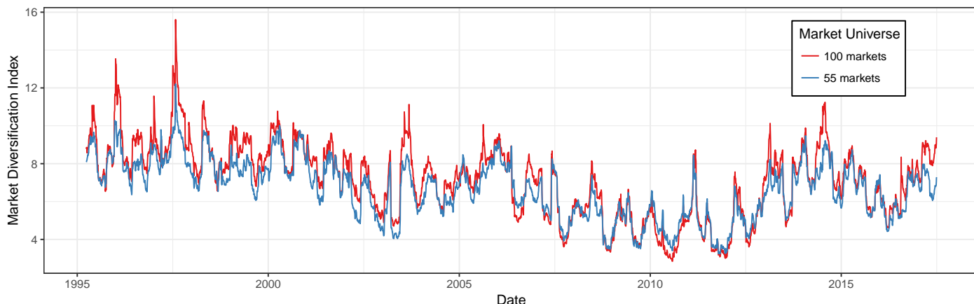
Figure 2. History of Market Diversification Index (MDI). The MDI has been relatively low since the financial crisis in 2008, with the exception of 2014-2015. Note that the index varies little between 55 and 100 markets.
