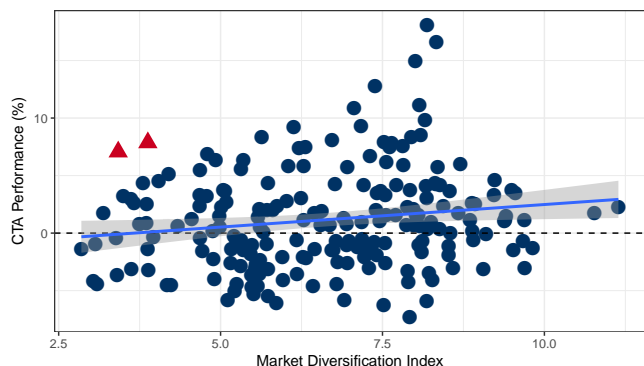
Figure 1. Since the creation of the SG CTA Index in 2000, CTA performance tends to be higher when the MDI takes larger values. The two outliers shown in triangles correspond to late 2008.
