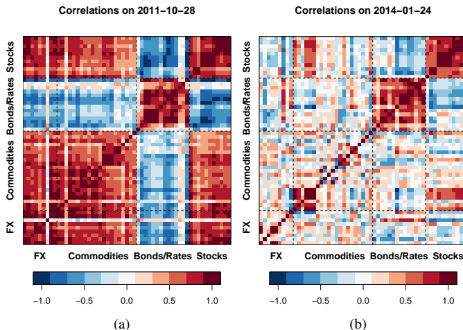
Figure 3. These heatmaps represent correlation matrices corresponding to low (a) and high (b) MDI levels.
